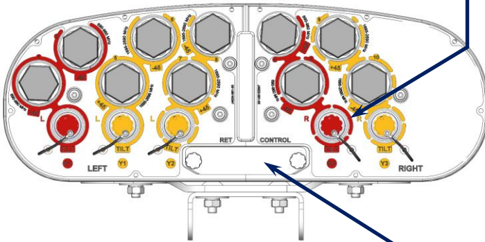
Location of the MDCU for RET control
